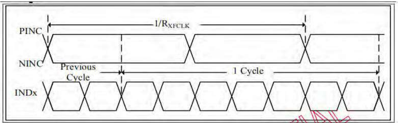
LVDS timing(1)
