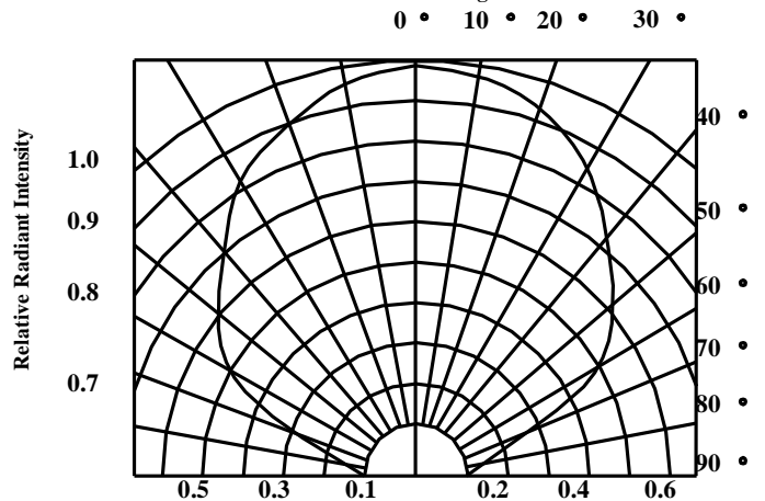
Radiation diagram
