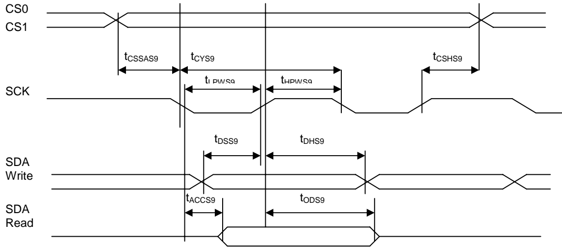
FIGURE 17: Serial Bus Timing Characteristics (for S9)
