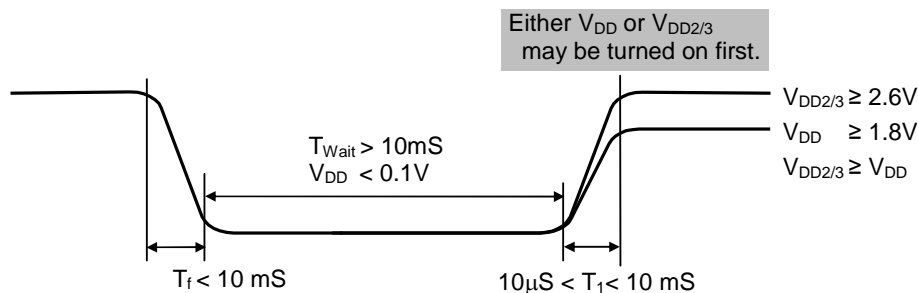
Figure 13: Delay allowance between V_{DD} and V_{DD2/3}
