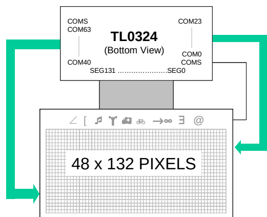
Figure 9-15. SHL = 0, ADC = 1
