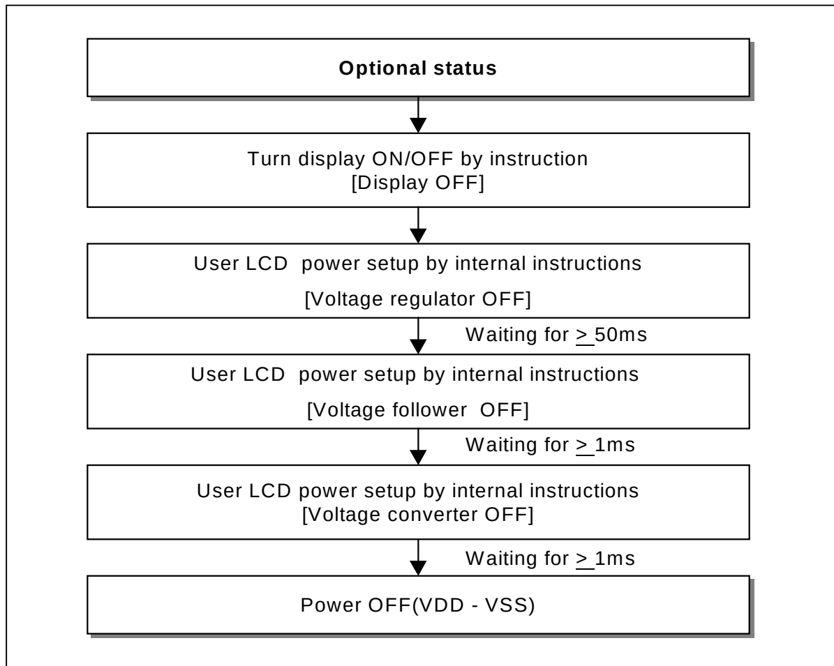
Figure 7-9. Power off.
