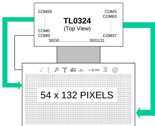
Figure 9-10. SHL = 0, ADC = 0
