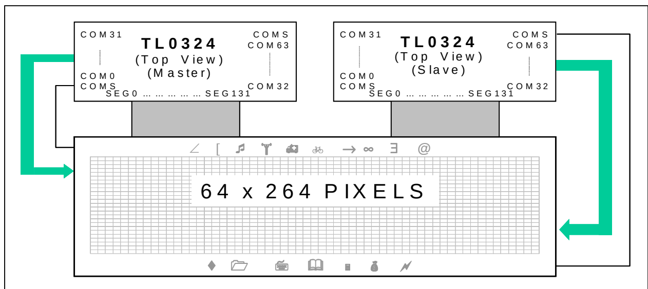
Figure 9-21. SHL = 0, ADC = 0
