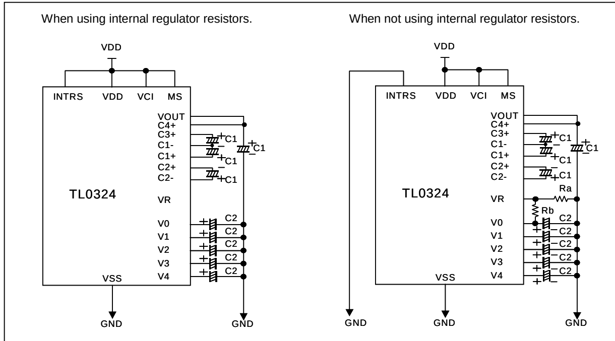
Figure 6-15. When using all LCD power circuits (VCI = VDD, 4-time, V/C: ON, V/R: ON, V/F: ON)
