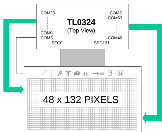
Figure 9-14. SHL = 0, ADC = 0
