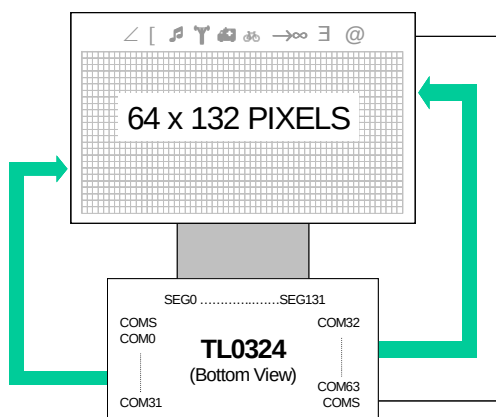
Figure 9-4. SHL = 1, ADC = 0
