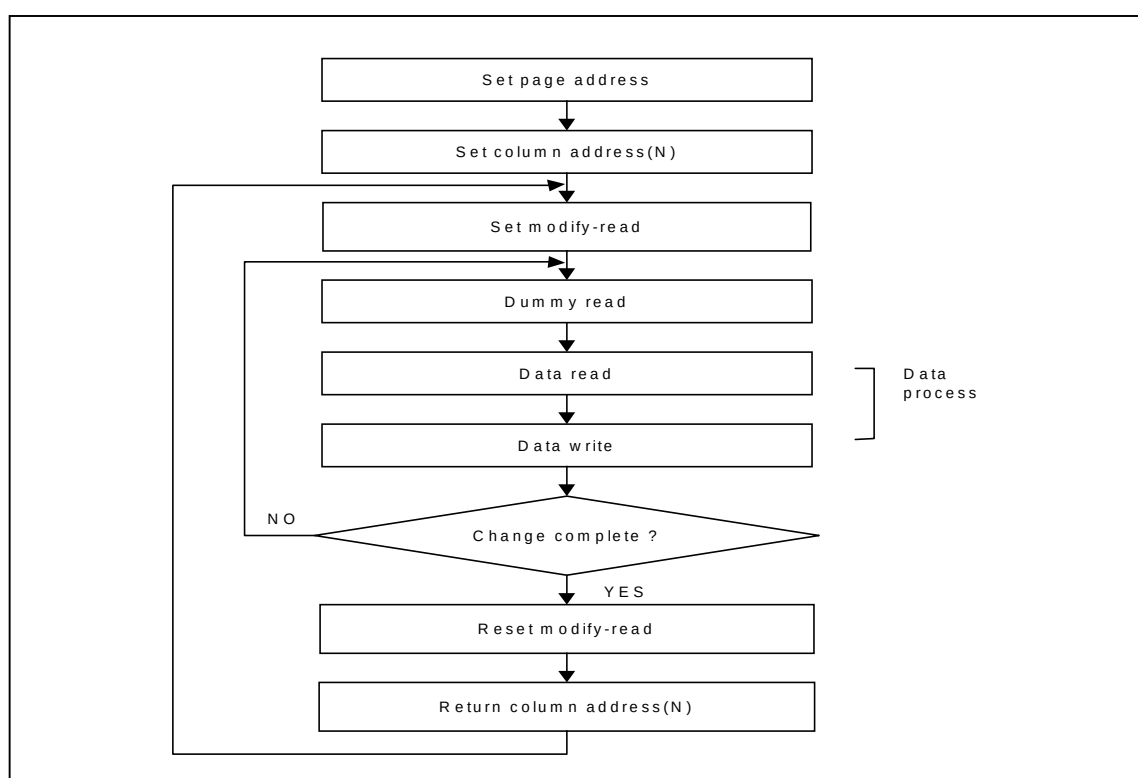
Figure 7-4. Sequence for cursor display
