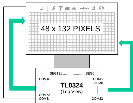
Figure 9-13. SHL = 1, ADC = 1
