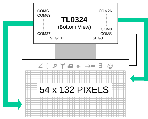
Figure 9-11. SHL = 0, ADC = 1
