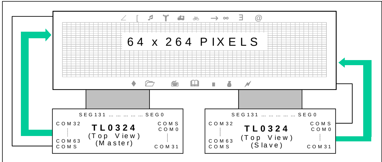
Figure 9-20. SHL = 1, ADC = 1
