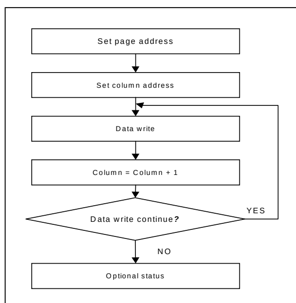
Figure 7-1. Sequence for writing display data
