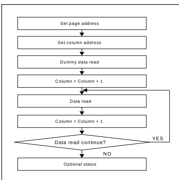
Figure 7-2. Sequence for reading display data
