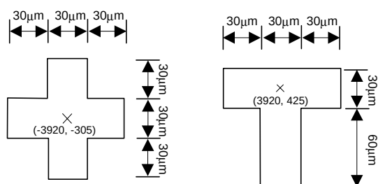
Figure 4-2. COG align key
