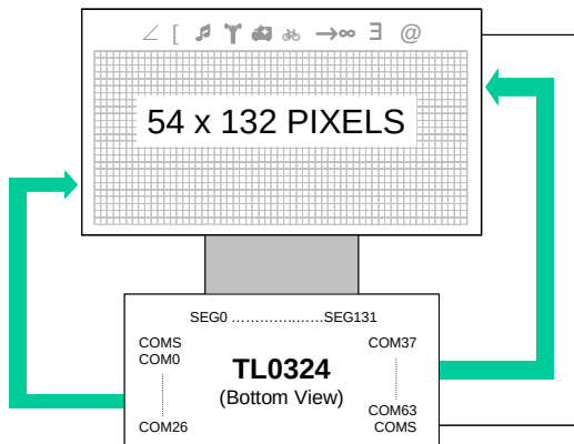
Figure 9-8. SHL = 1, ADC = 0
