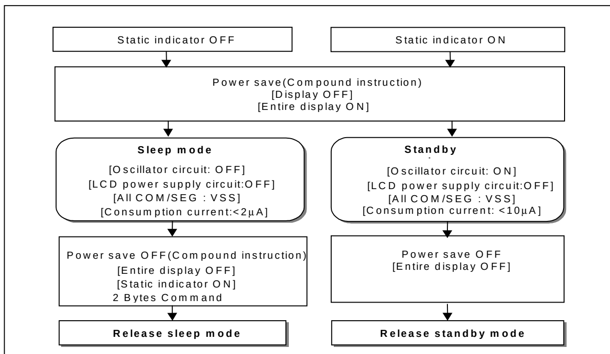
Figure 7-5. Power save routine
