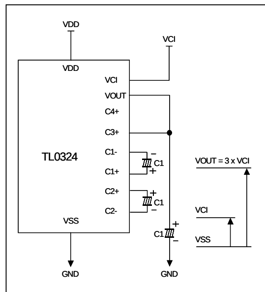
Figure 6-10. Three times boosting circuit
