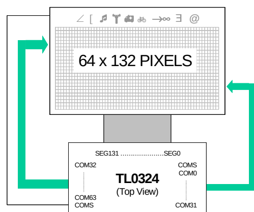
Figure 9-5. SHL = 1, ADC = 1
