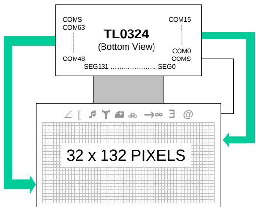
Figure 9-19. SHL = 0, ADC = 1
