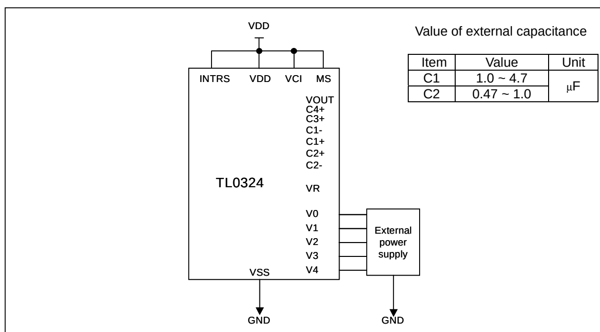
Figure 6-18. When not using any LCD power supply circuits (VCI = VDD, V/C: OFF, V/R: OFF, V/F: OFF)
