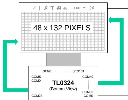
Figure 9-12. SHL = 1, ADC = 0
