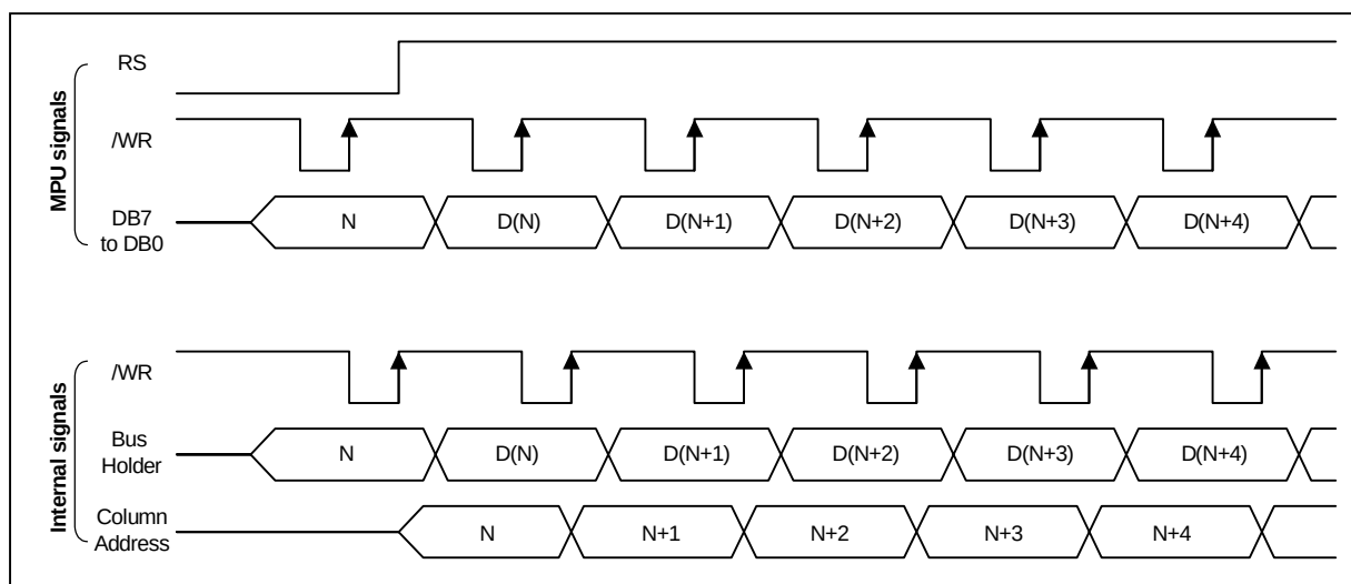
Figure 6-2. Write timing
