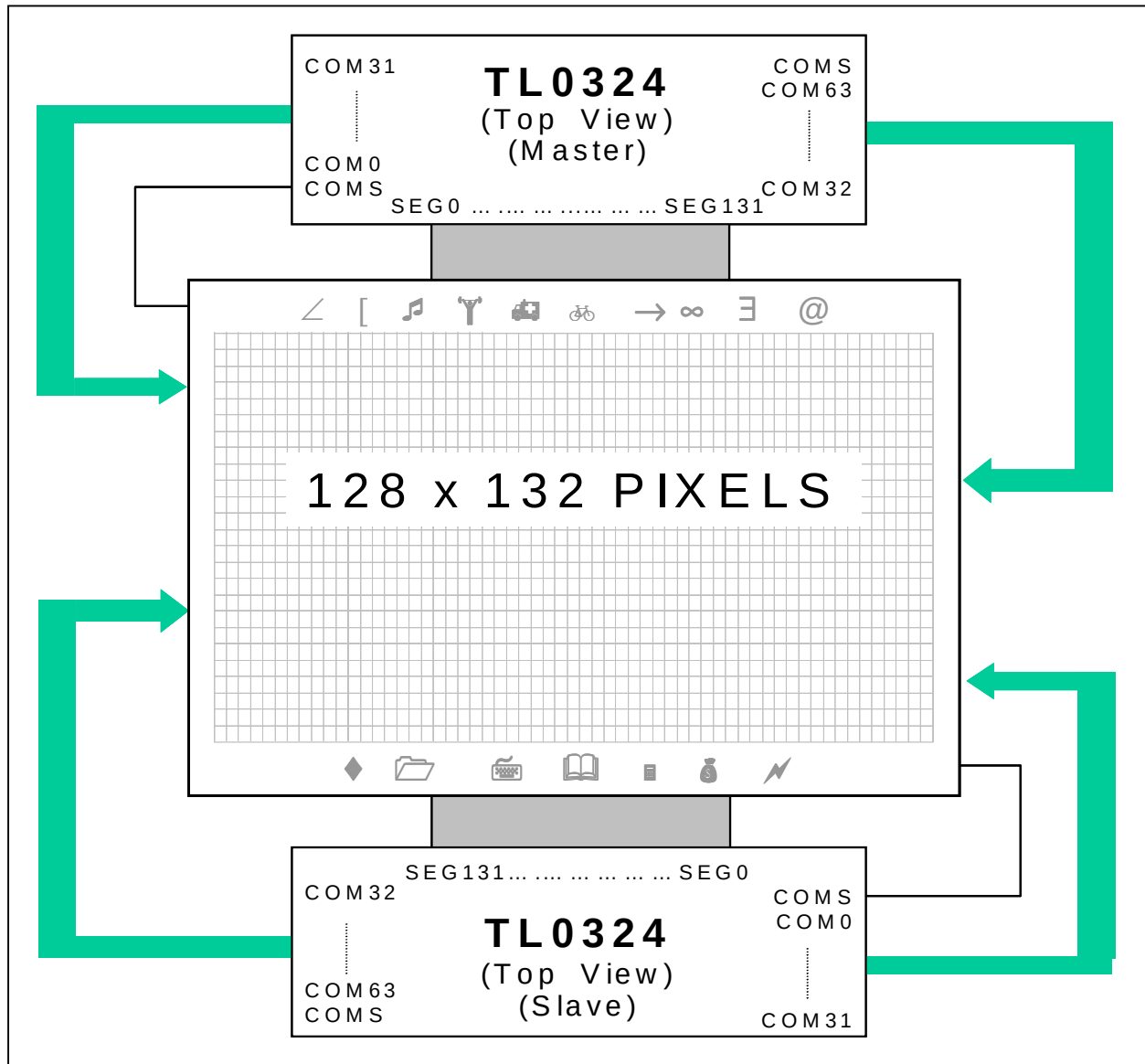
Figure 9-22. 130COM (128COM + 2COMS) x 132SEG
