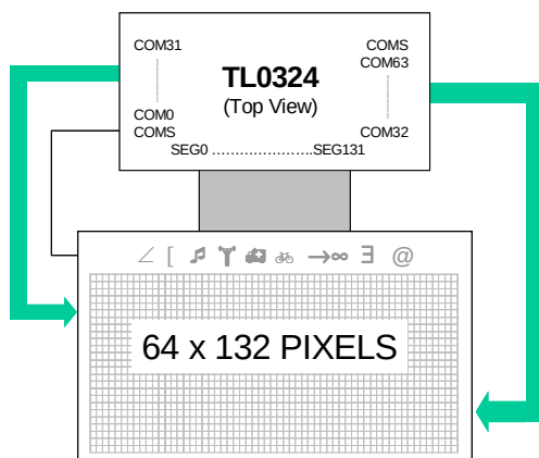
Figure 9-6. SHL = 0, ADC = 0
