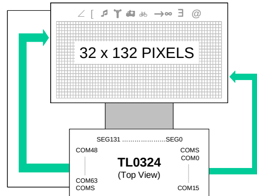
Figure 9-17. SHL = 1, ADC = 1
