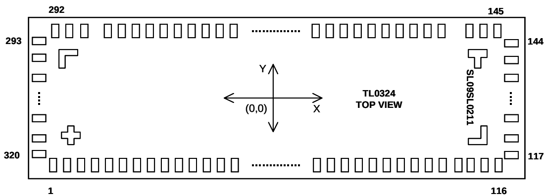
Figure 4-1. Chip configuration
