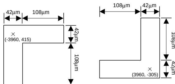
Figure 4-3. ILB align key
