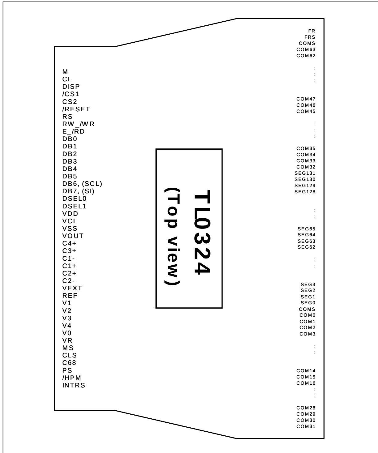
Figure 9-23. TCP pin layout
