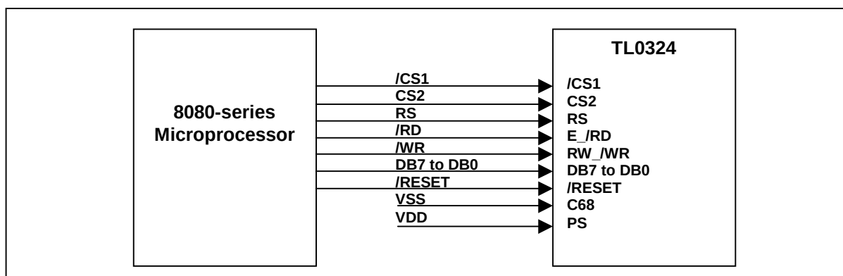
Figure 9-3. 8080-series MPU Interface (PS = "H", C68 = "L")
