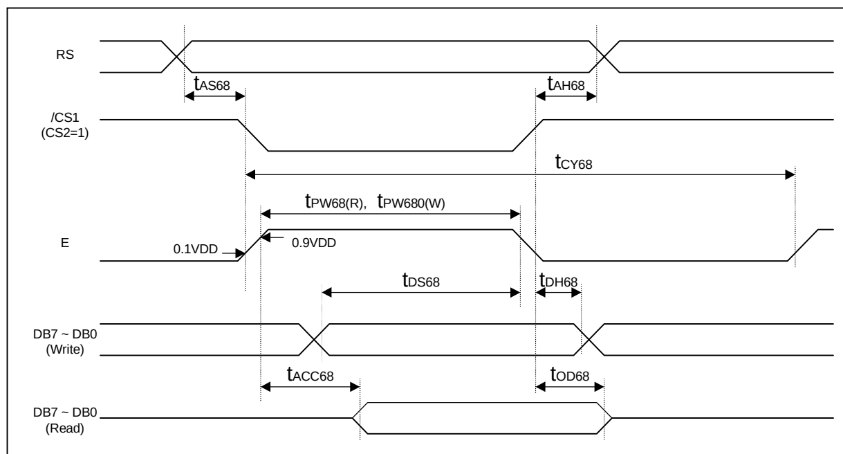
Figure 8-5. Read / write timing chart (6800-series MPU)
