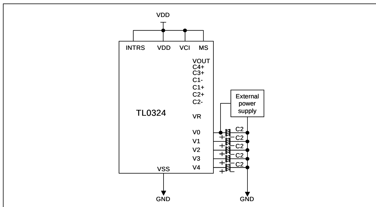
Figure 6-17. When using some LCD power circuits (VCI = VDD, V/C: OFF, V/R: OFF, V/F: ON)
