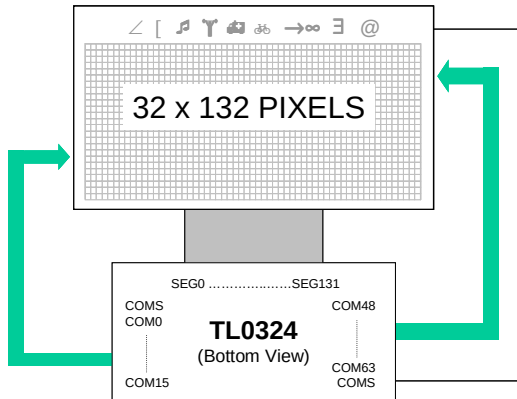
Figure 9-16. SHL = 1, ADC = 0
