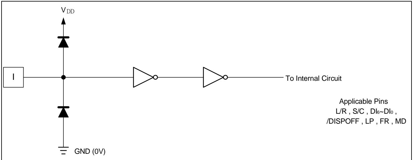
Figure 6-1 Input Circuit (1)
