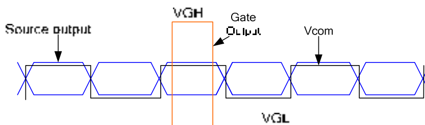
Fig.17.5 Voltage Output to TFT LCD Panel
