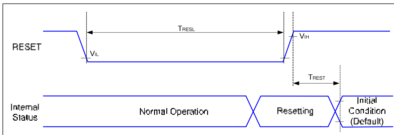
Fig. 12.4 Reset timing
