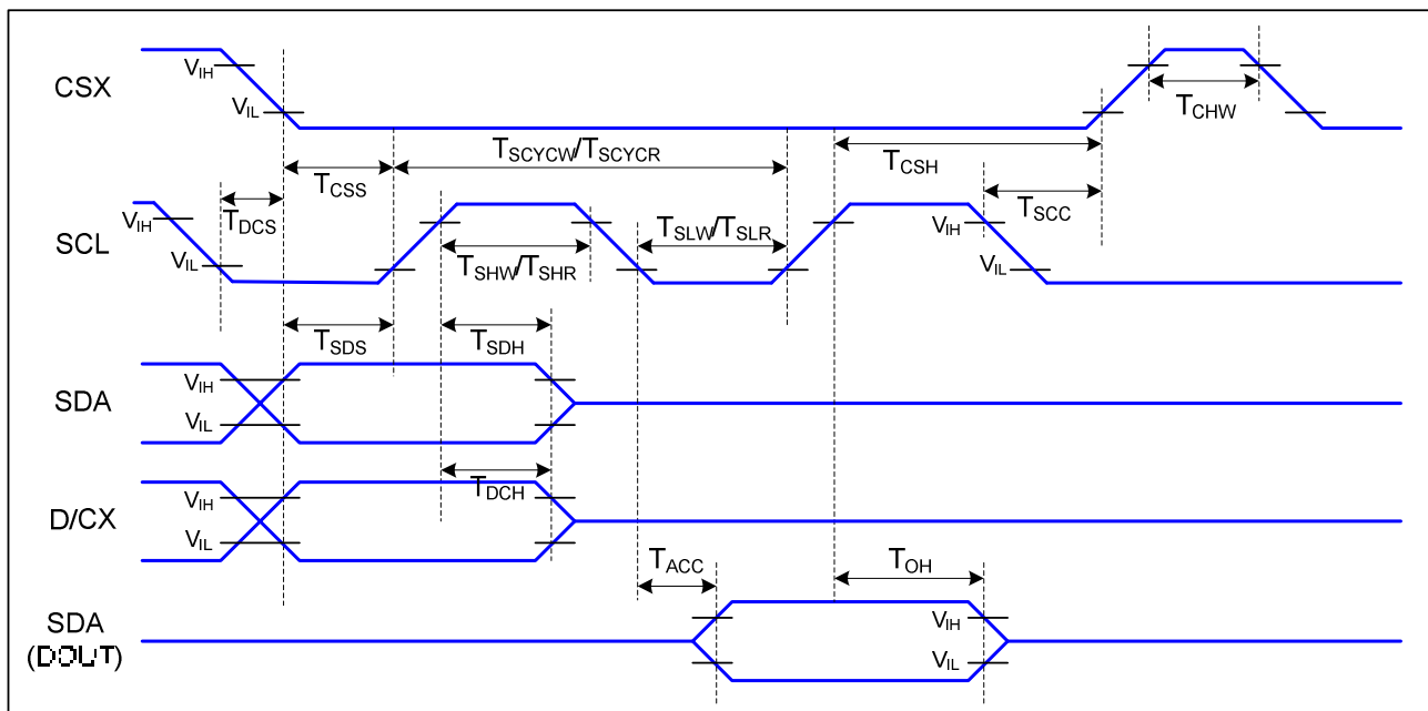
Figure 8.4.1 4-line serial interface timing T_a = 25^\circ\text{C} , V_{DDI} = 1.65 \sim 3.7\text{V} , V_{DD} = 2.3 \sim 4.8\text{V}
