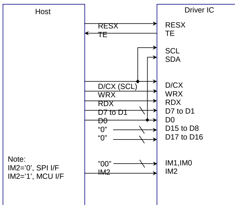
Fig 13.3.1 8080 Series MCU Interface for 8-bit data bus
