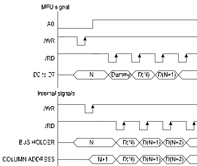
Figure 13 Read Timing
