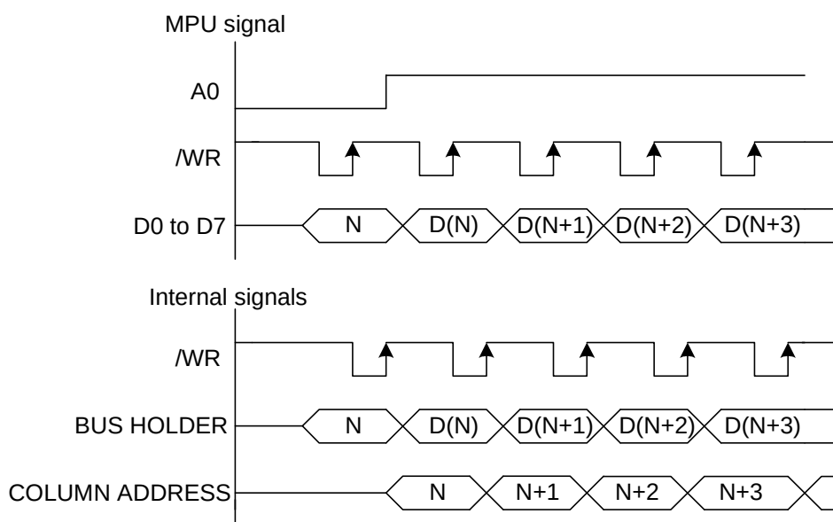
Figure 12 Write Timing
