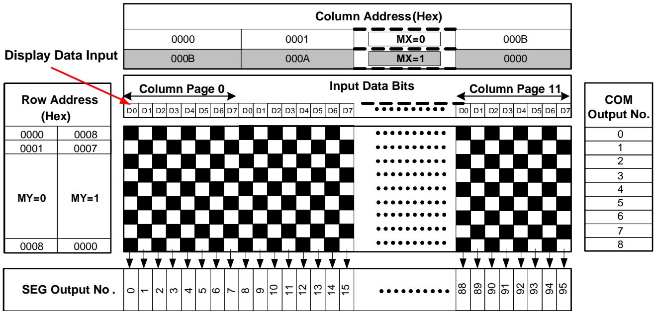
Fig. 42 Data Format and DDRAM Structure
