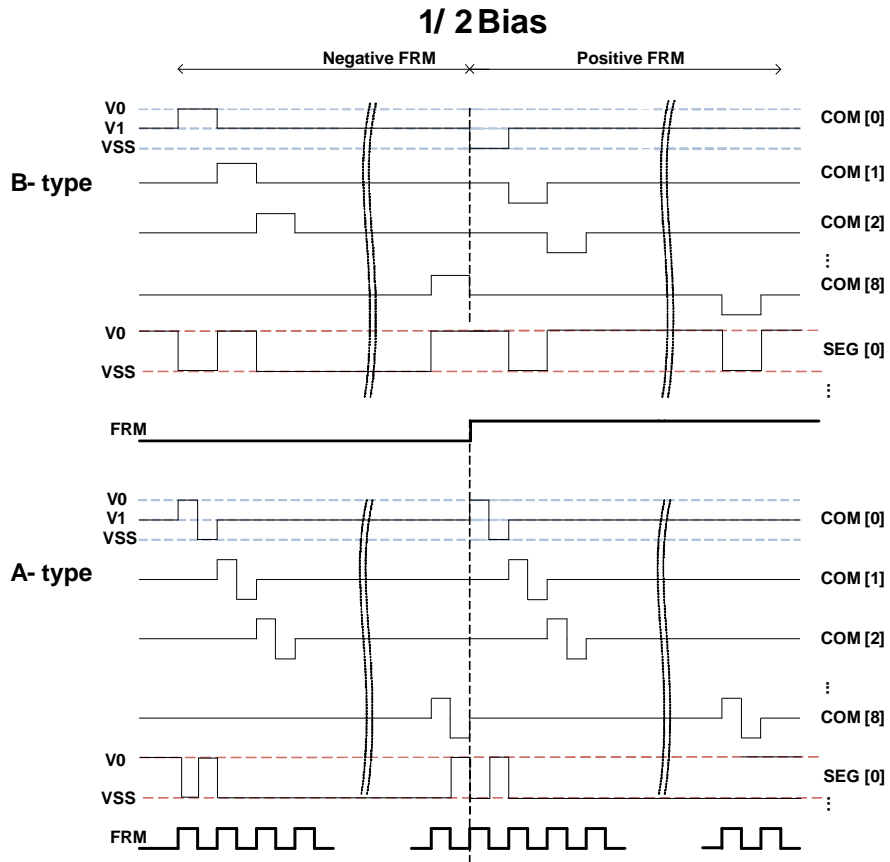
Fig. 198 A-type & B-type of 1/2 Bias waveform
