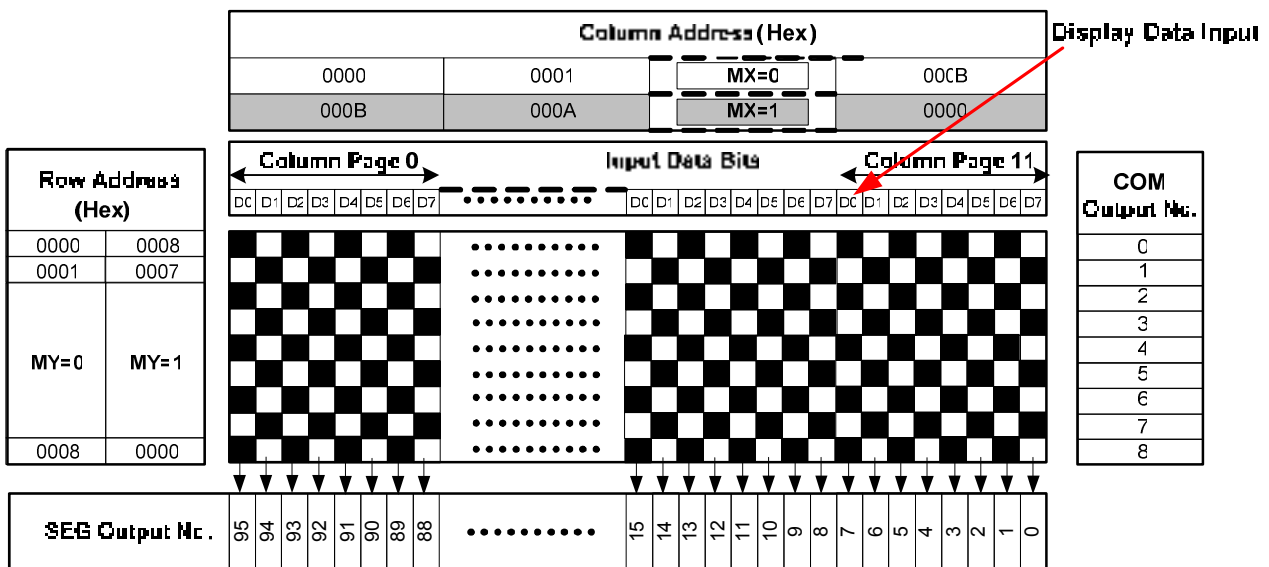
Fig. 53 Transferred DDRAM Map
