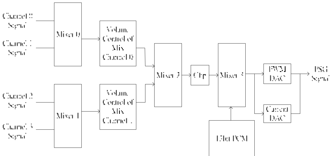
FIGURE 10-2 PSG Four Channel Mixer Structure Block
