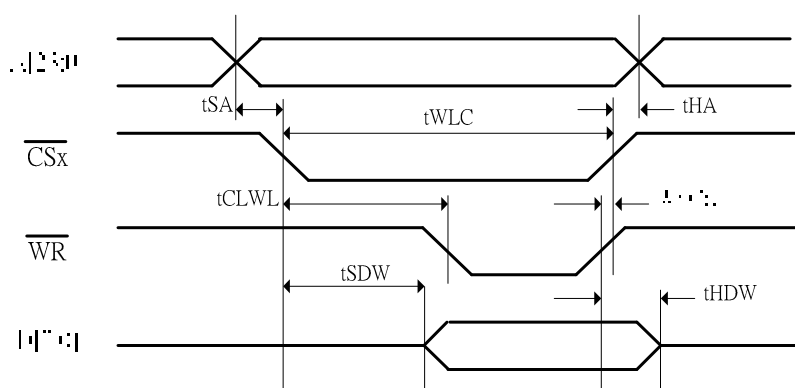
FIGURE 22-2 External Write Timing Diagram
