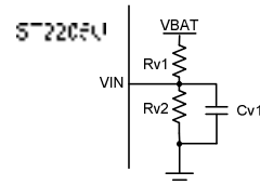
FIGURE 20-2 Application of LVD (2)
