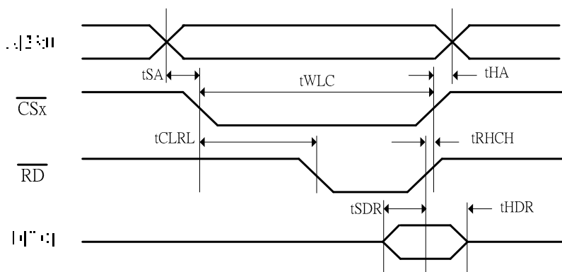
FIGURE 22-1 External Read Timing Diagram
