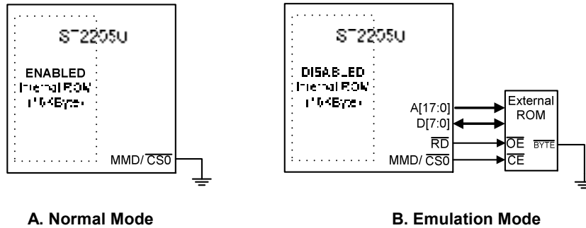
FIGURE 8-1 Connections Of MMD/CS0
