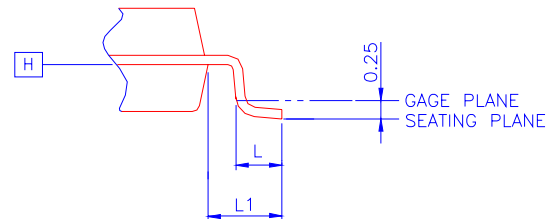
DETAIL A
