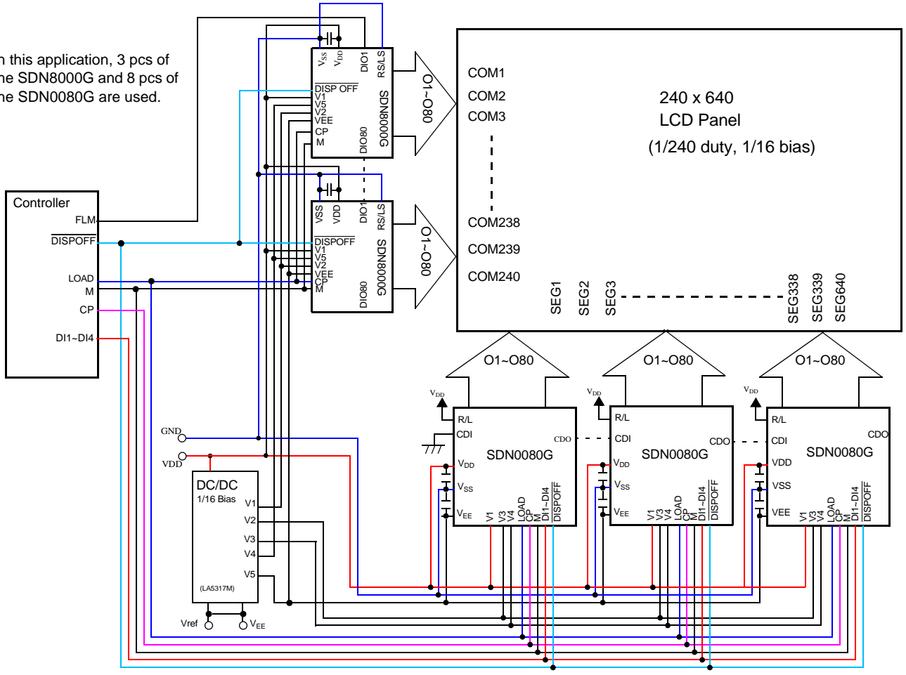
Fig.9 Typical application circuit
