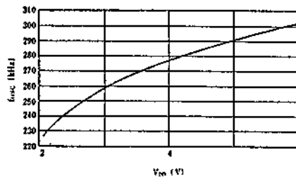
Note 11) Supply Voltage vs Oscillating Frequency
