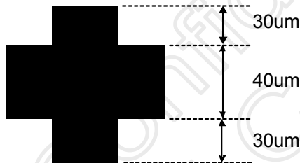
Alignment Mark1
