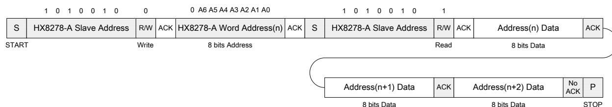
Figure 6.26: I2C format
