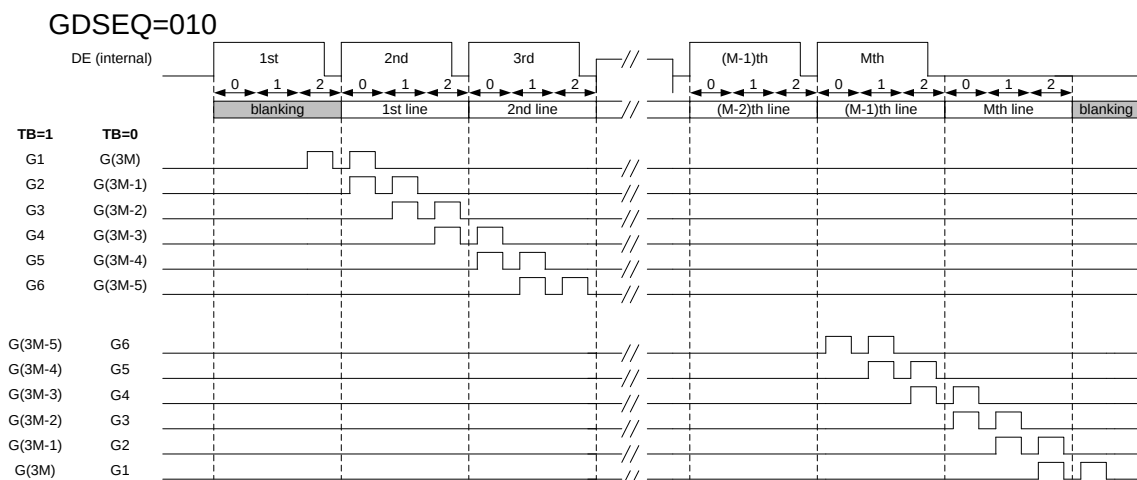
Figure 5.6: Gate scan type 2
