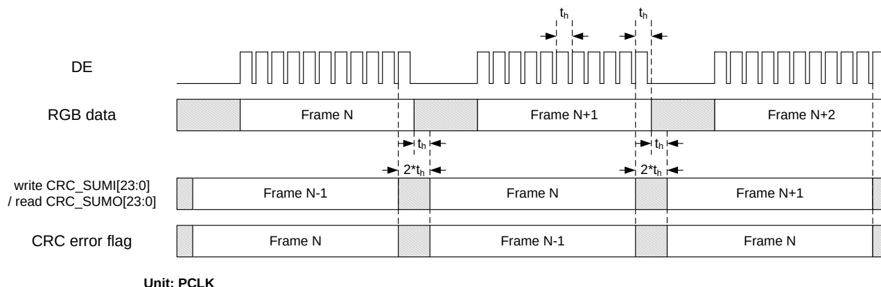
Figure 6.13: CRC timing
