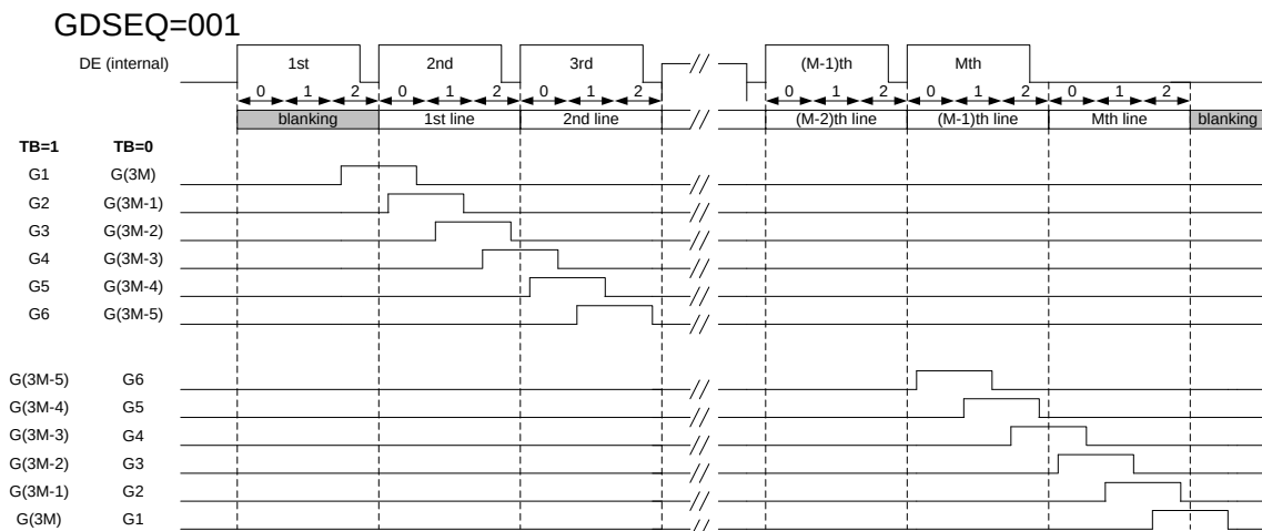
Figure 5.5: Gate scan type 1
