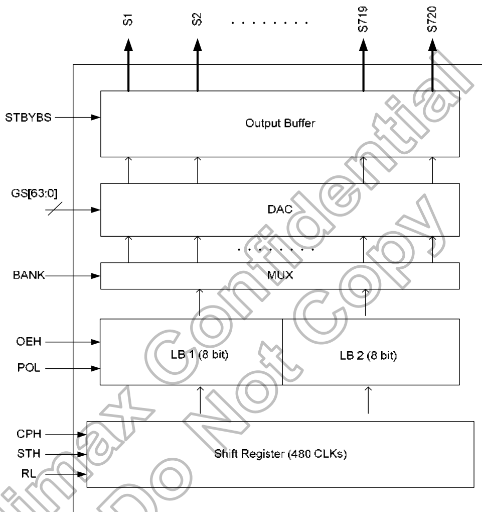
Figure 7.6 Source Block
