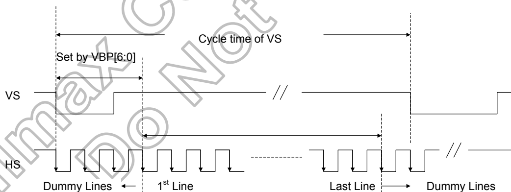
Figure 8.3 Vertical Data
