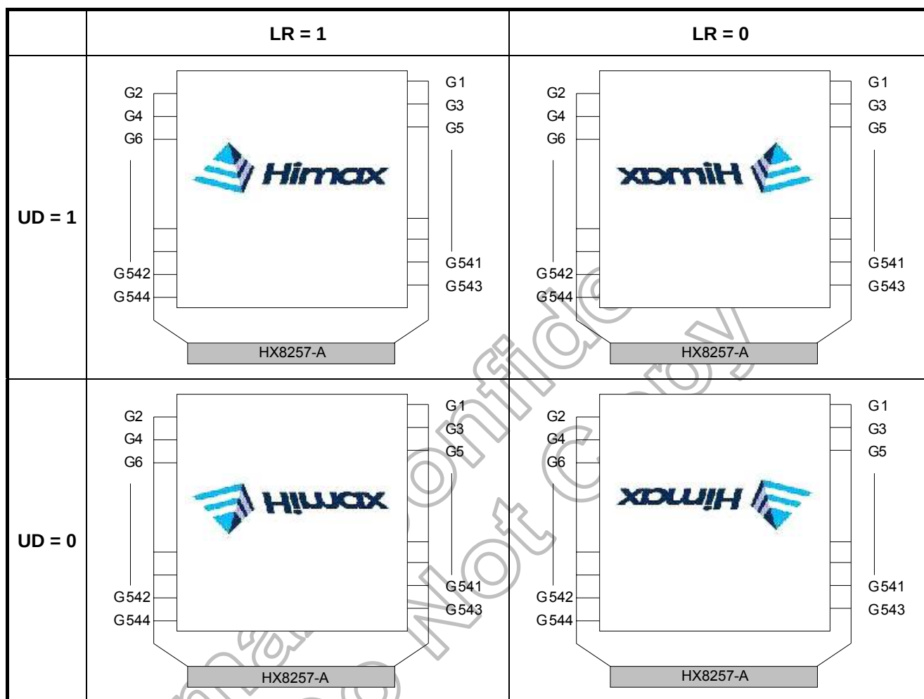
Figure 7.13 LR/UD Function
