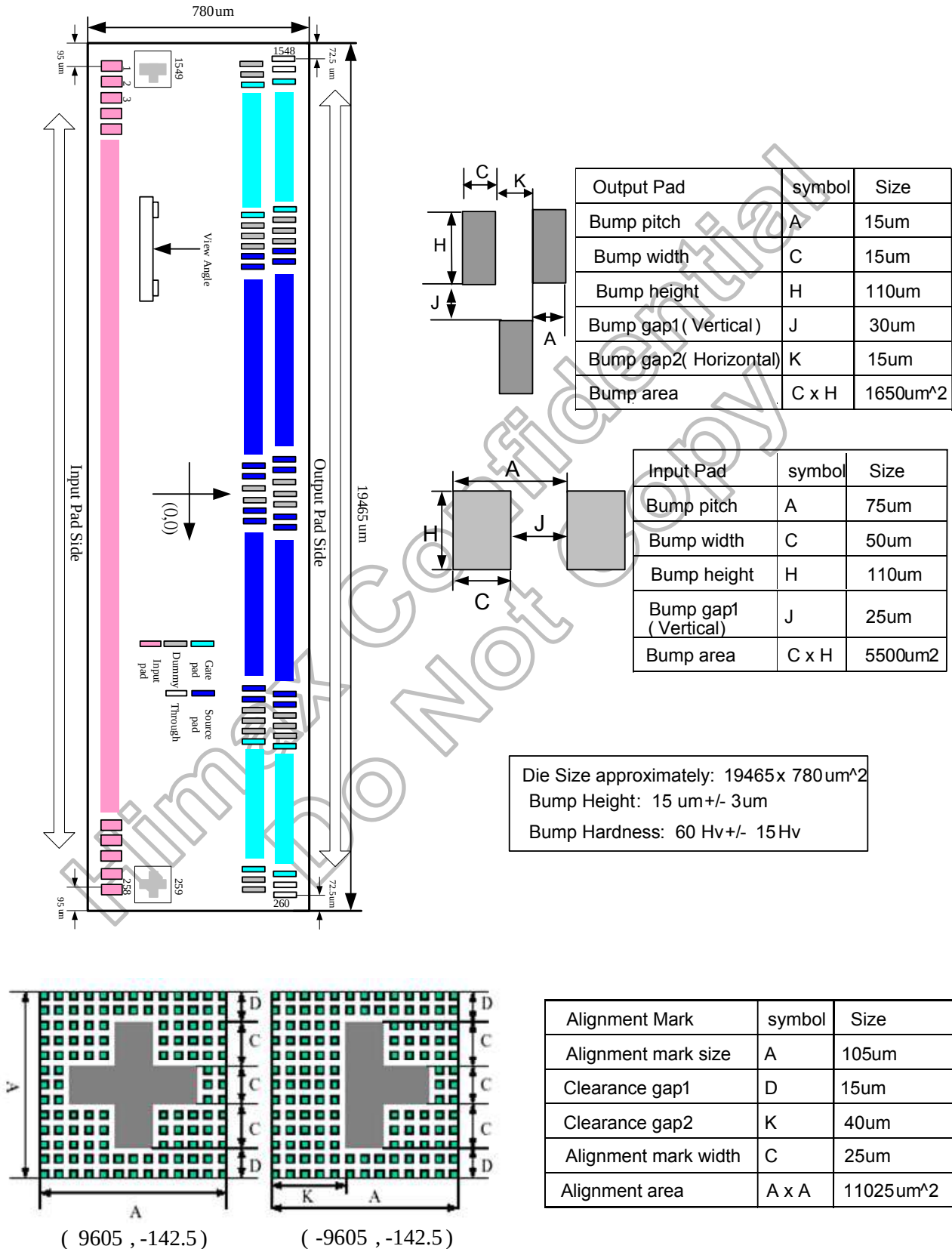
Figure 4.1 HX8257-A Die Floor Plan (Bump Face UP)
