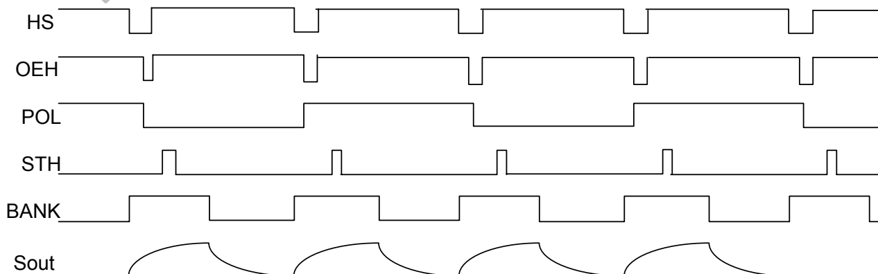
Figure 7.7 Source Sequence
