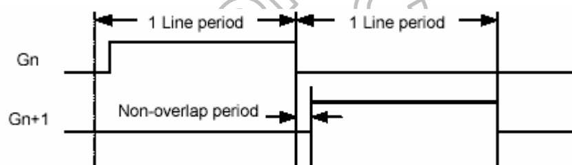
Figure 8. 10 NO Timing Diagram
