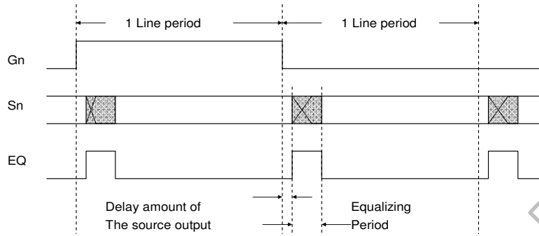
Figure 8. 11 EQ Timing Diagram
