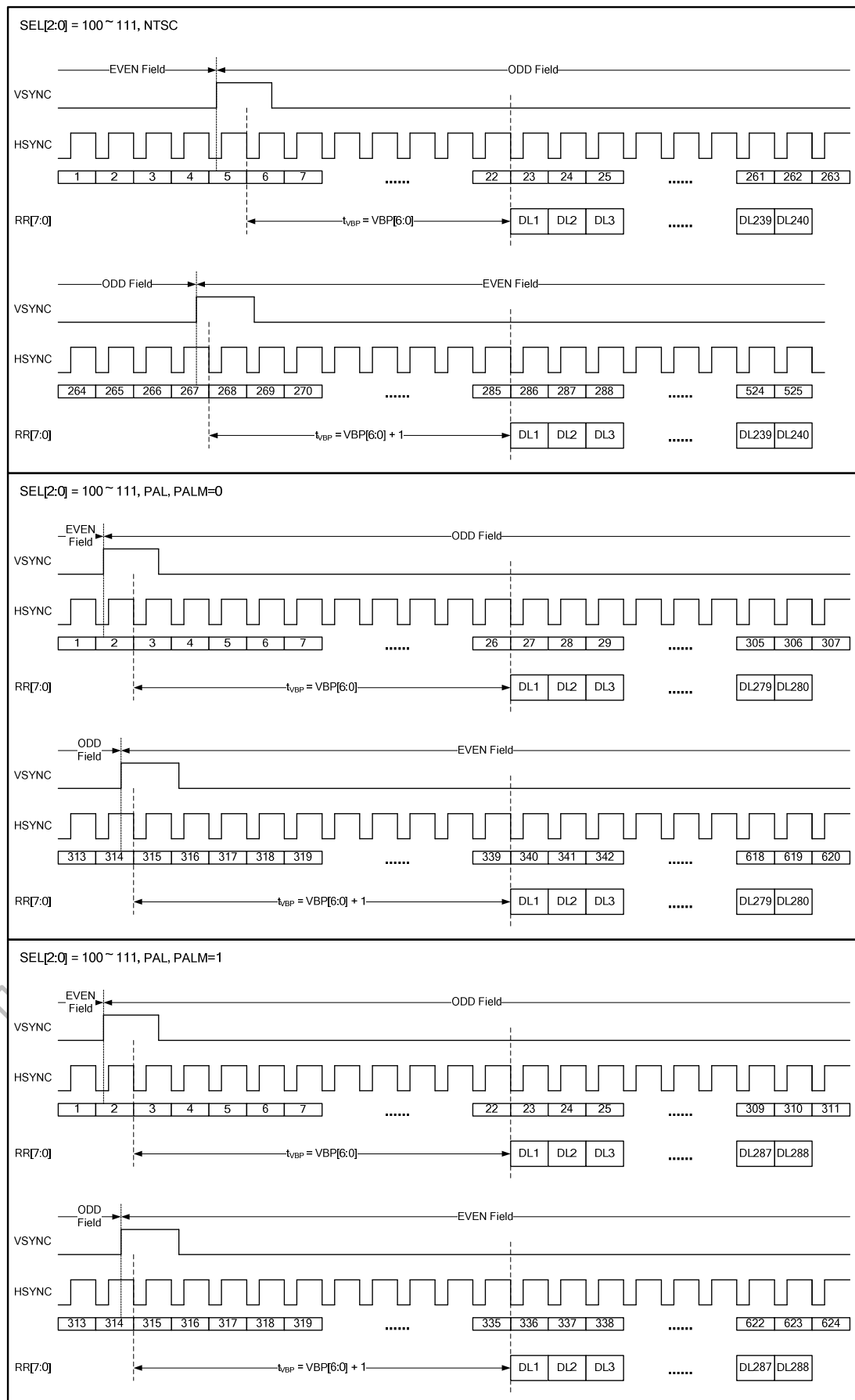
Figure13. 8 CCIR601 Vertical Timing
