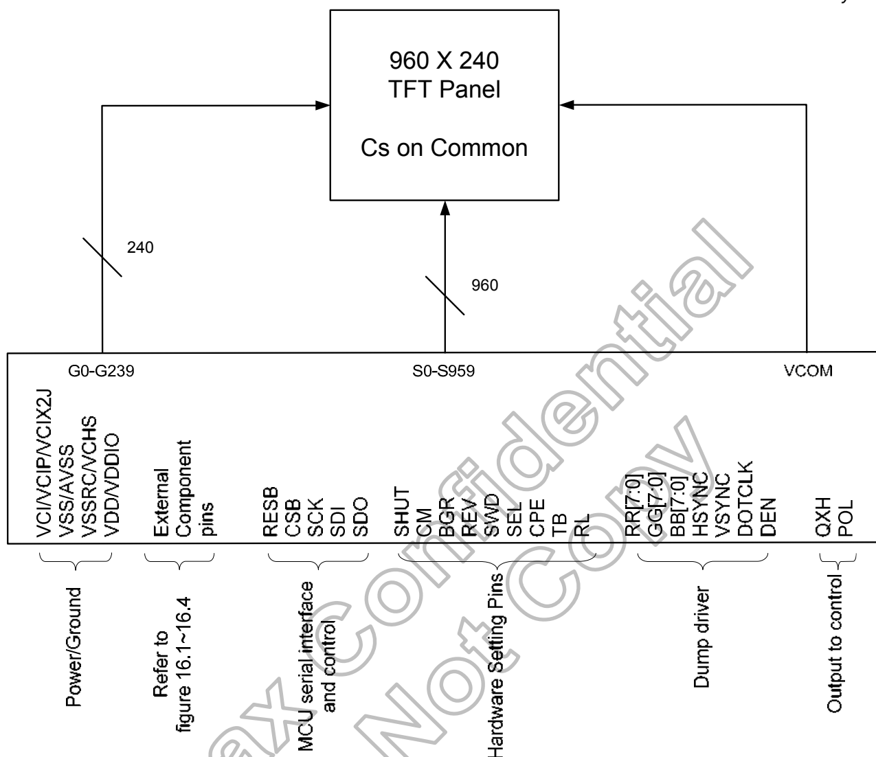
Figure 15.5 Panel Connection Example
