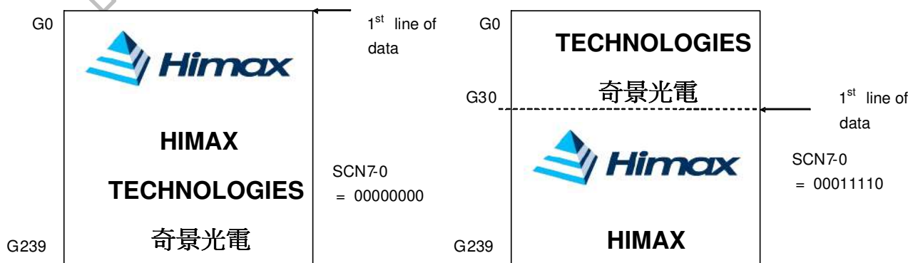
Figure 8. 15 Gate scan display position
