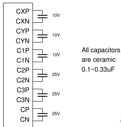
Figure 15.1 Booster Capacitors
