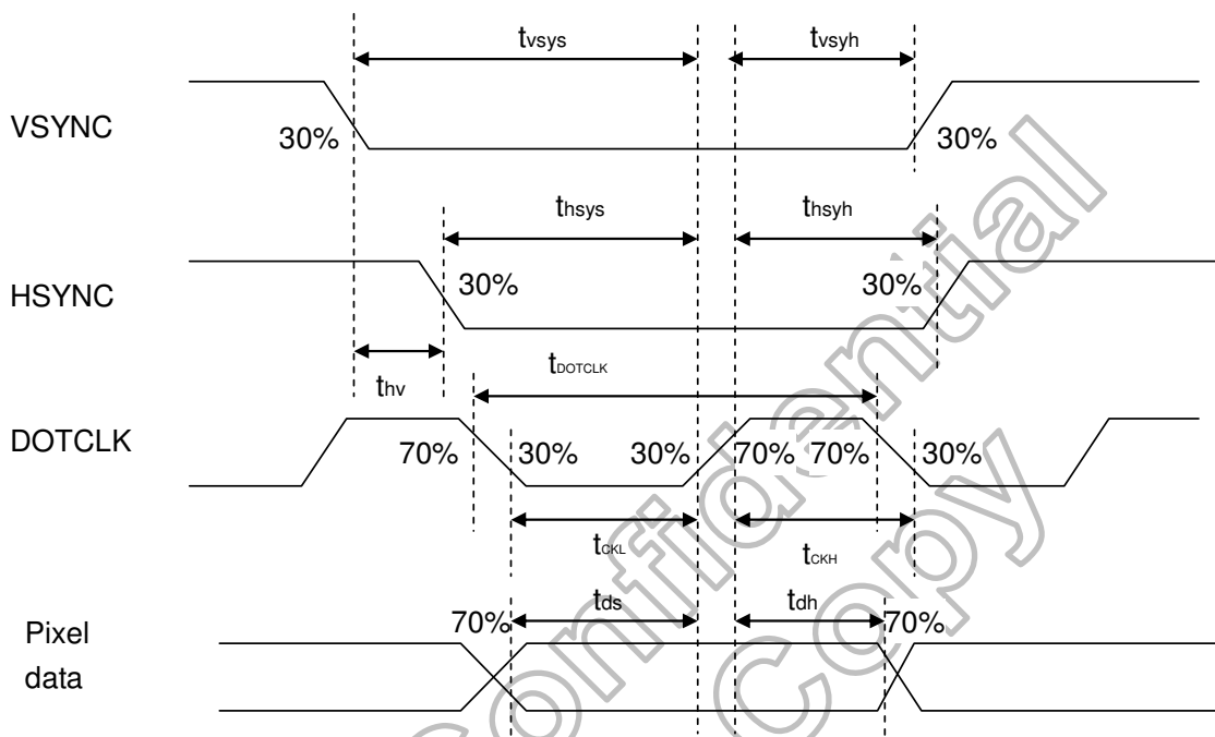
Figure13. 1 Pixel Timing
