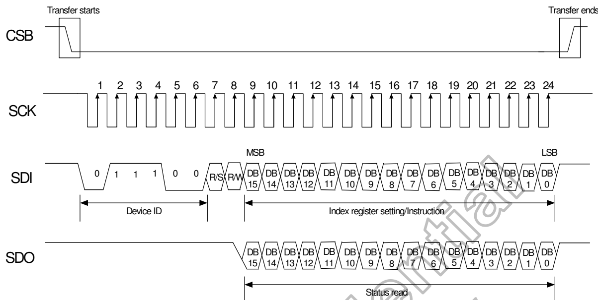
Figure 6. 1 SPI Timing
