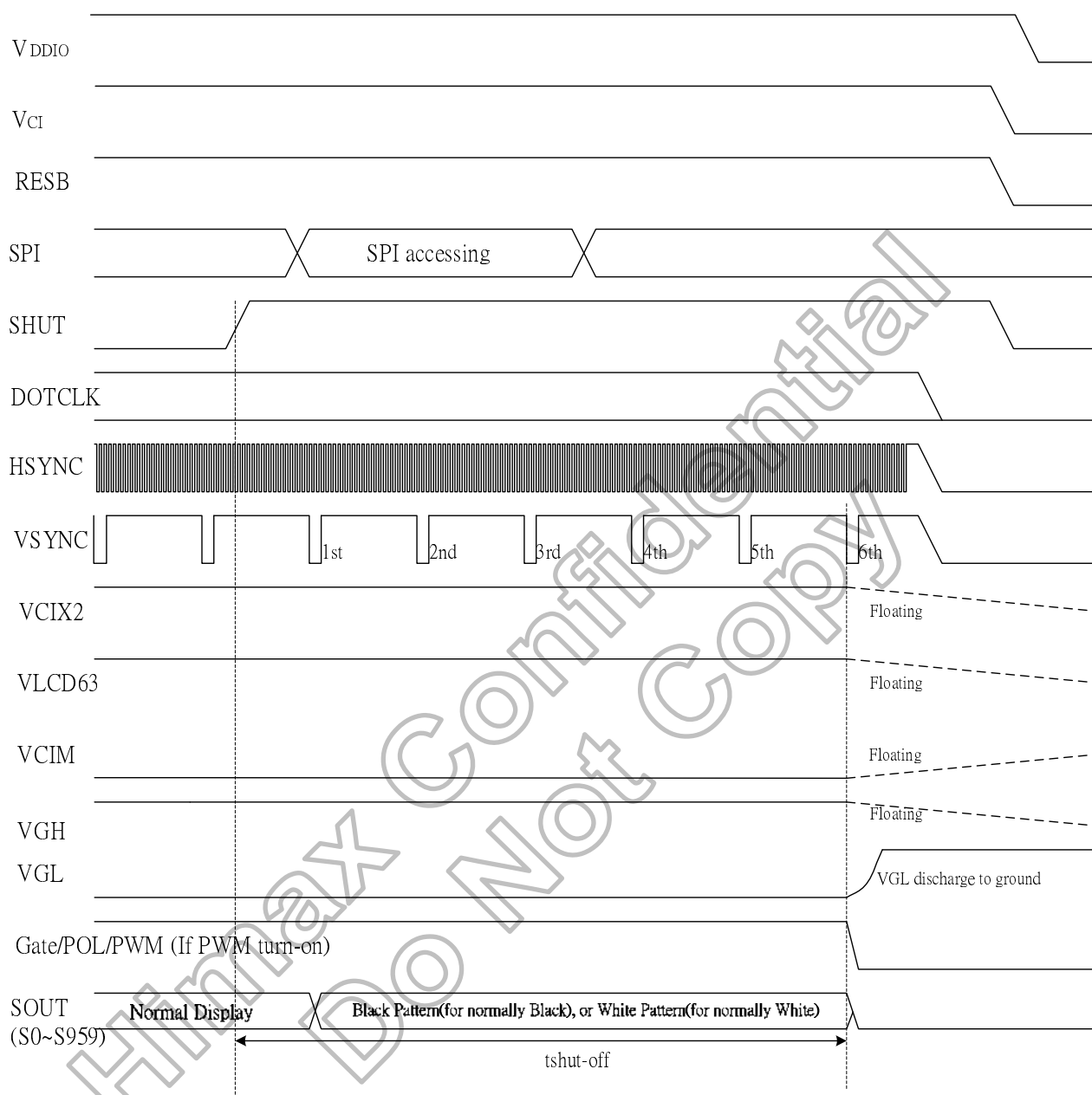
Figure13. 12 Power Down Sequence
