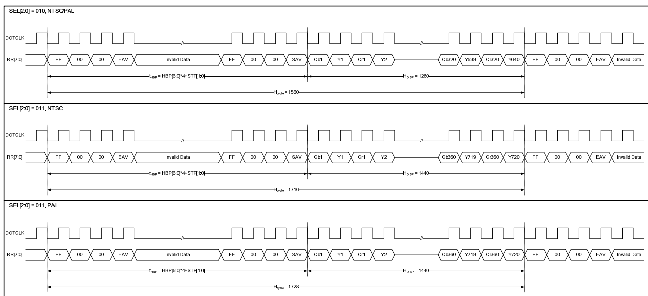
Figure13. 9 CCIR656 Horizontal Timing
