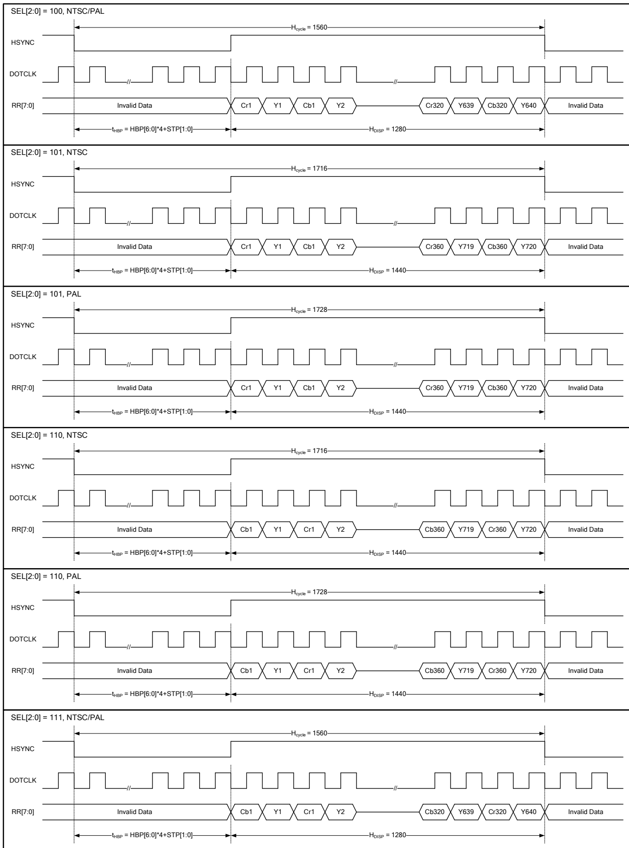
Figure13. 7 CCIR601 Horizontal Timing
