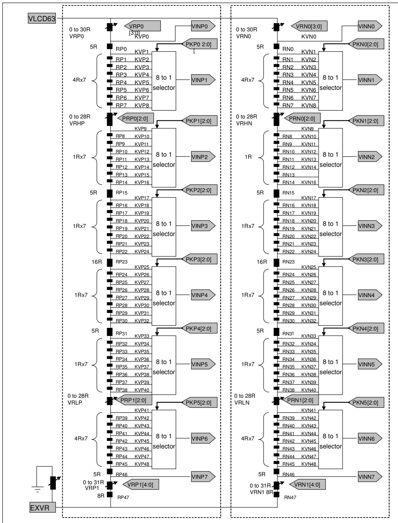
Figure 10. 3 Resistor Ladder for Gamma Voltages Generation
