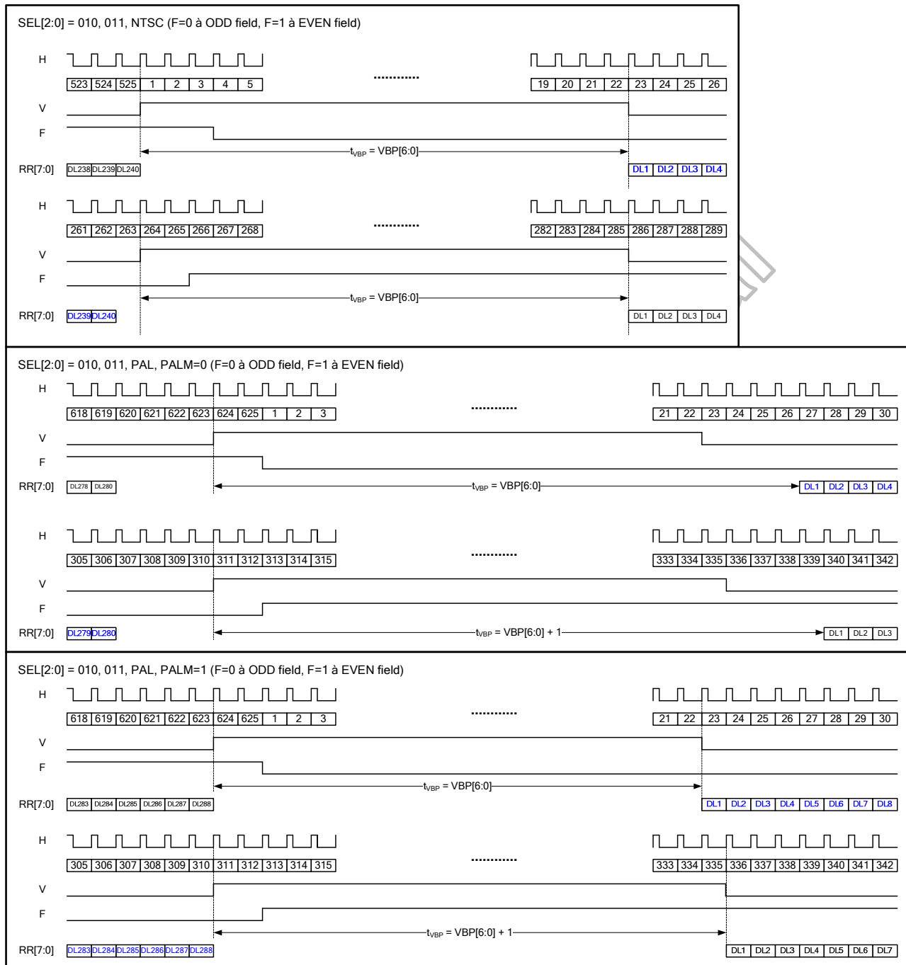
Figure13. 10 CCIR656 Vertical Timing
