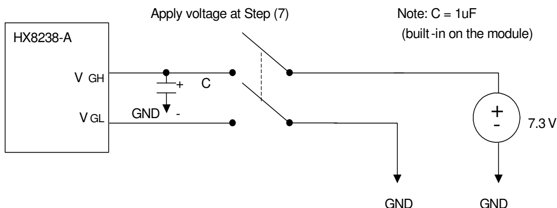
Figure 9. 2 OTP Programming Circuitry
