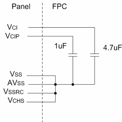
Figure 15. 4 Panel and FPC Connection
