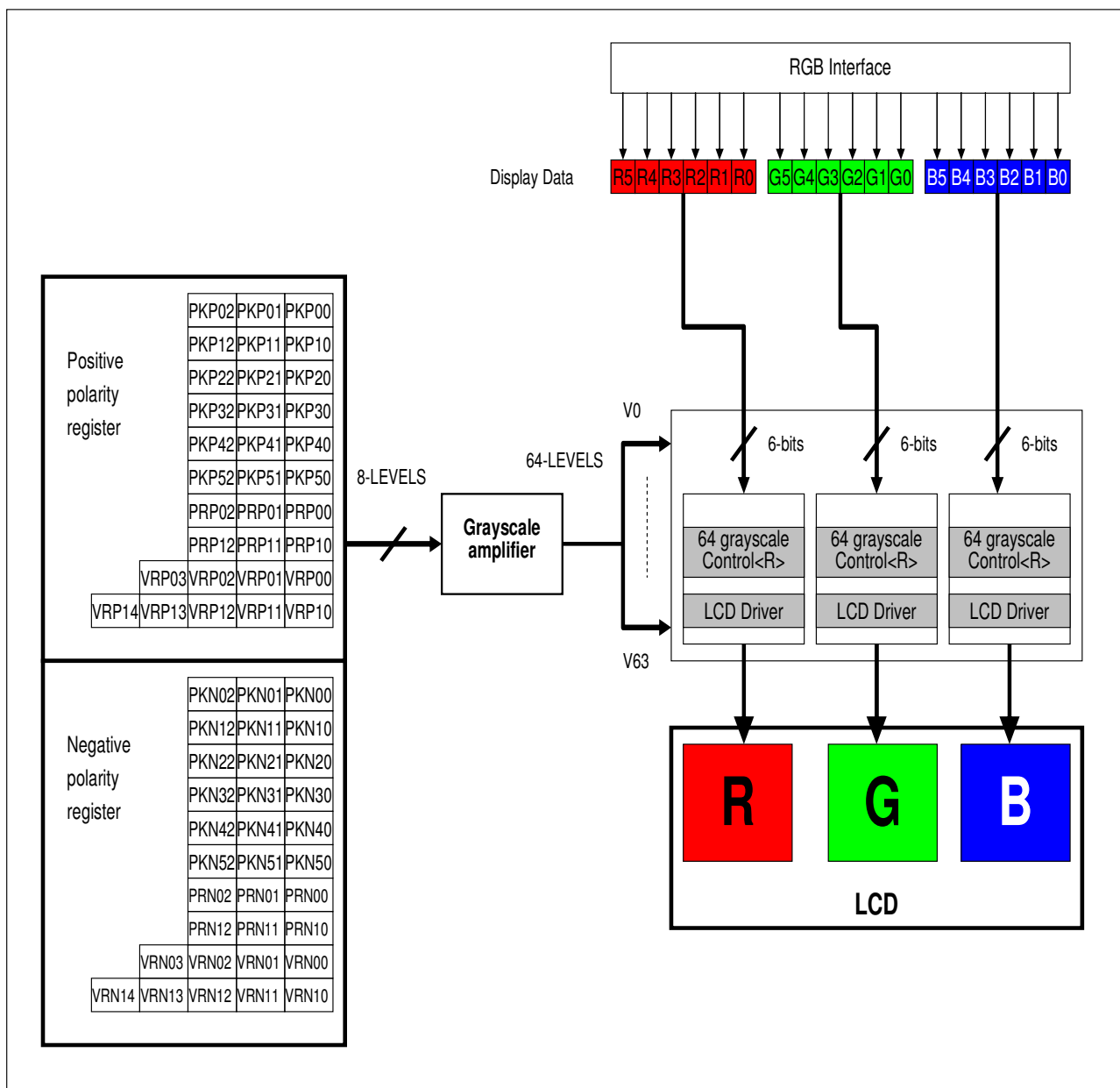
Figure 10. 1 Grayscale Control Block
