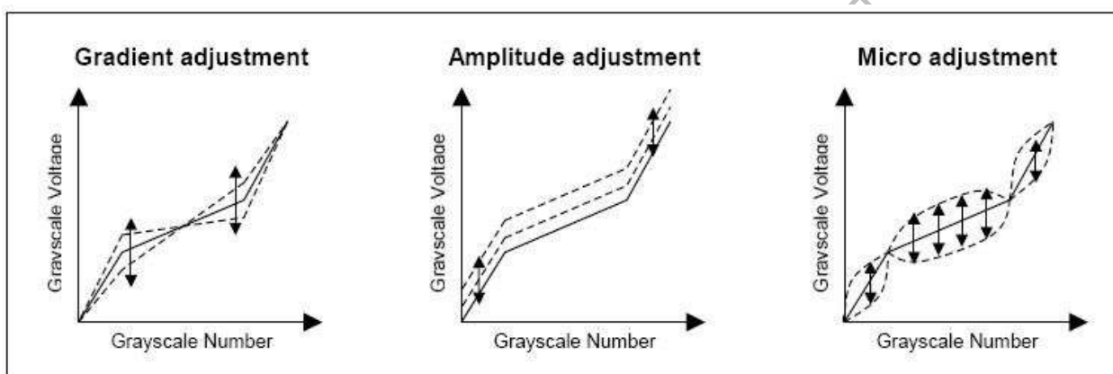
Figure 10. 4 Gamma Adjustment Function
