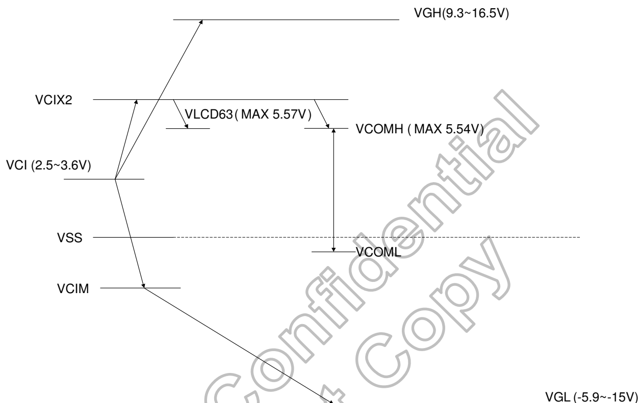
Figure 14. 1 LCD Driving Voltage Relationship
