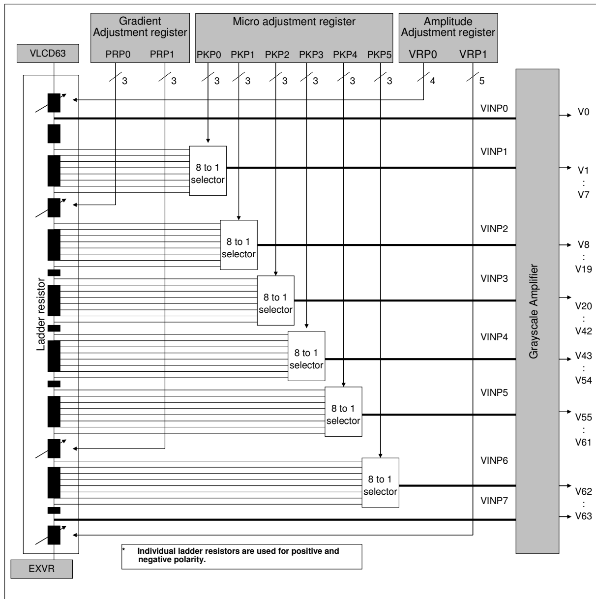
Figure 10. 2 Grayscale Amplifier
