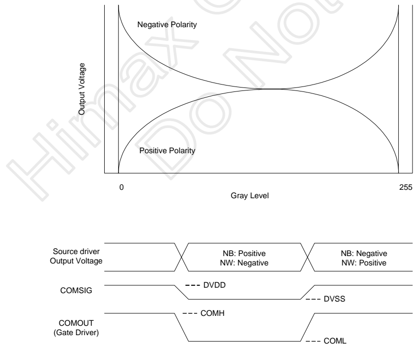
Figure 6. 4 Relationship between NB and NW output polarity
