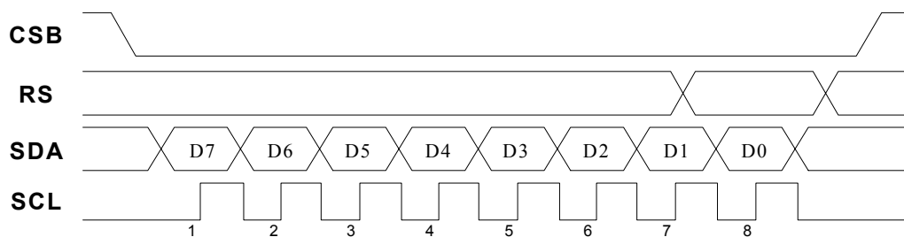
Figure 4. 4-Wires type Serial Interface
