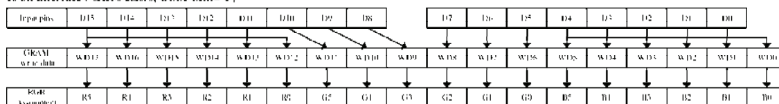
16 bit interface (65,536 colors, COM_SEL='0')
