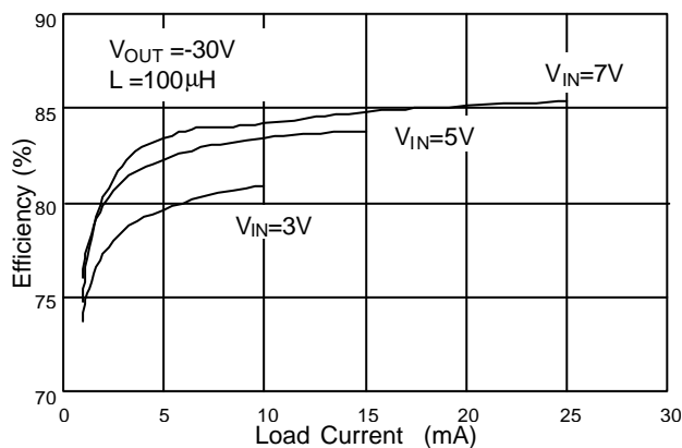
Fig. 9 Efficiency vs. Load Current
