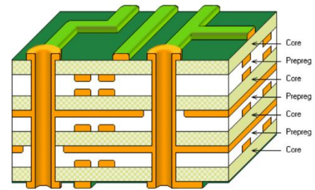
8-layer PCB Stack-up
