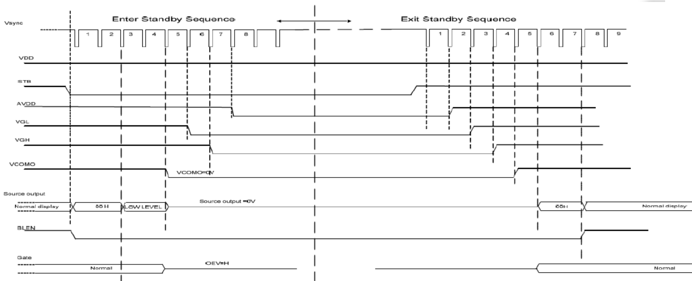
Enter and Exit Standby Mode timing chart
