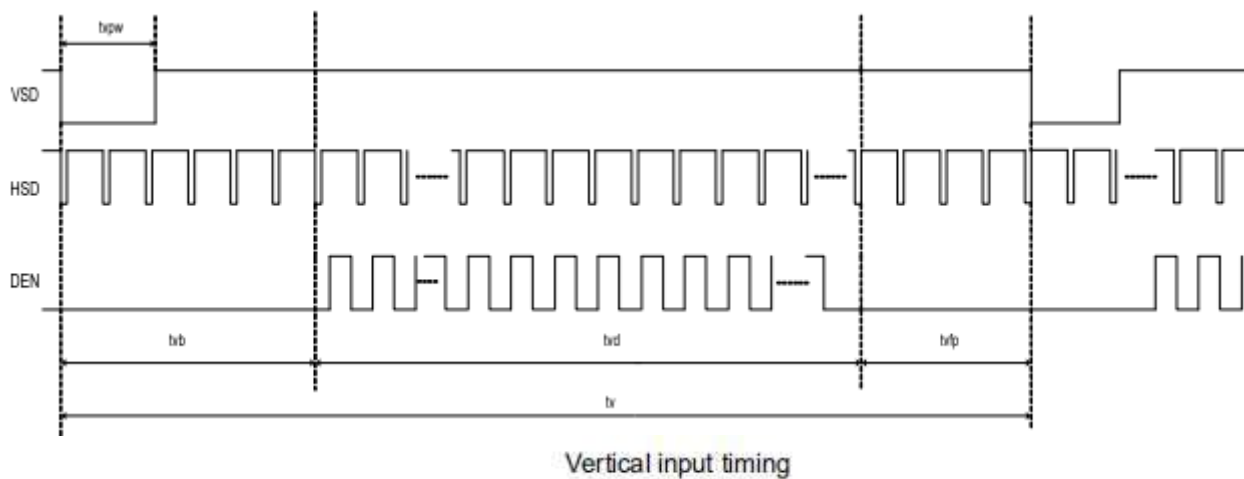
8-bit LVDS Input Timing chart
