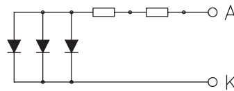
Backlight Circuit
