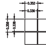
LCD DOTS DETAIL SCALE 20:1
