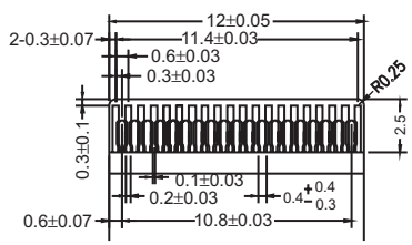
DETAIL B(S=3:1)
