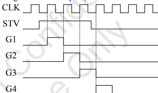
■Long Start Pulse Input (More Than 2 CLK Period)
