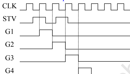
■Dual Start Pulse Input
