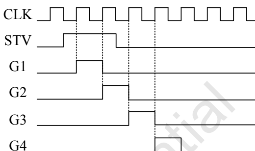
■Long Start Pulse Input (2 CLK Period)
